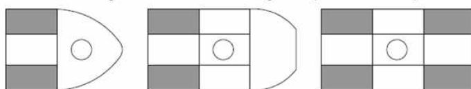
Fig 5.7 Loading Pattern with Scanting Draft
